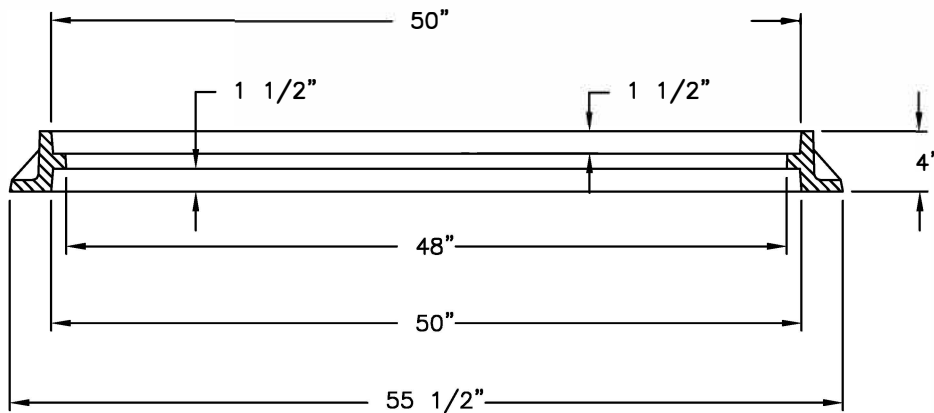
FRAME SECTION
