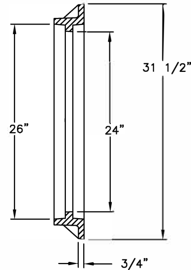
FRAME SECTION
